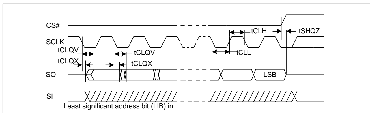
Figure41. Output Timing
