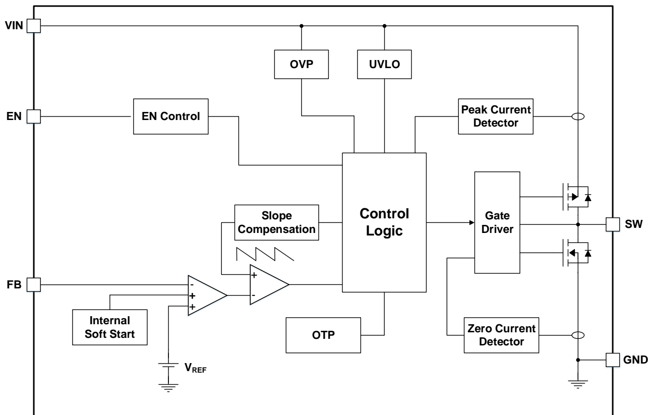
Figure 9. GD30DC1103 Functional Block Diagram
