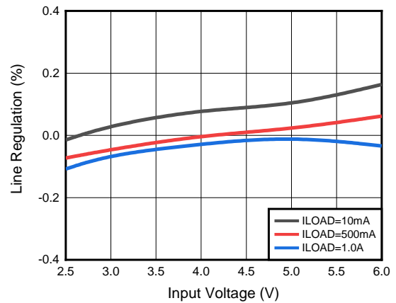
Figure 15. Line Regulation ( V_{OUT} = 1.2\text{V} )
