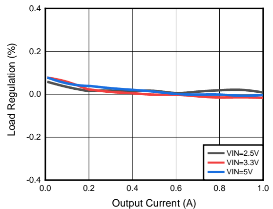
Figure 17. Load Regulation ( V_{OUT} = 1.8\text{V} )
