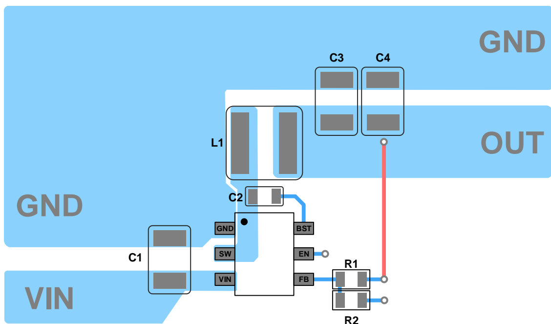
Figure 32. Typical GD30DC1314-I06 Example Layout
