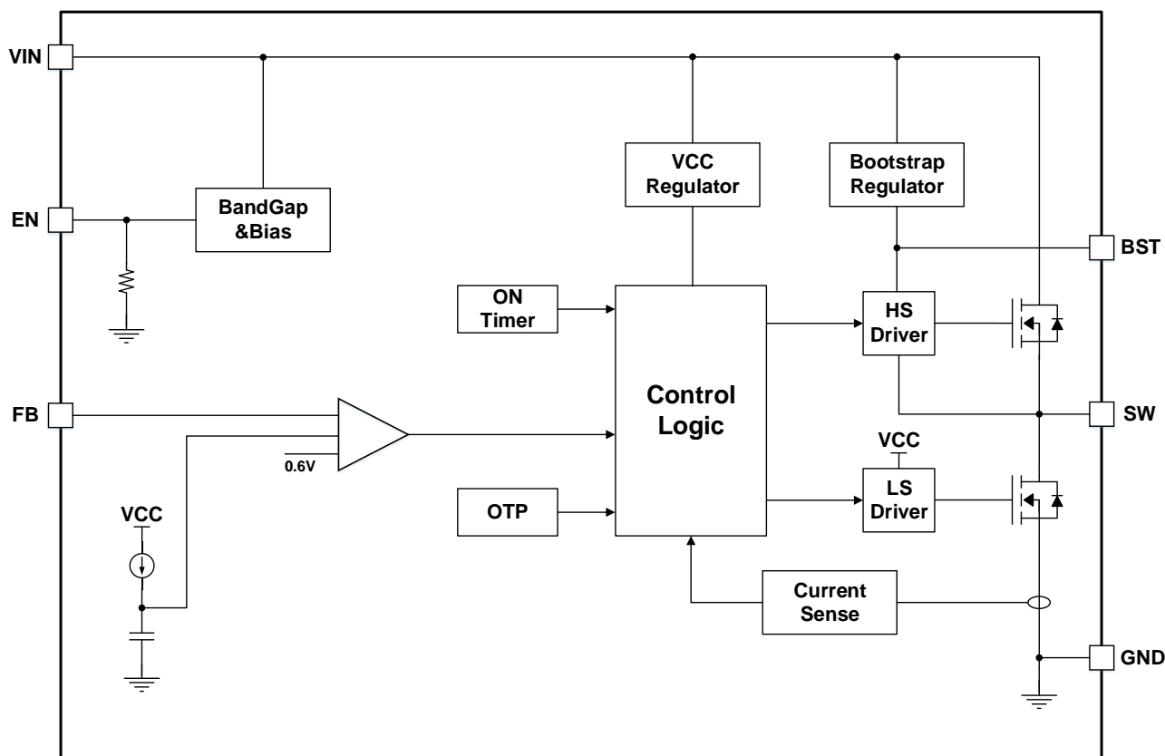
Figure 7. GD30DC1314-I06 Functional Block Diagram
