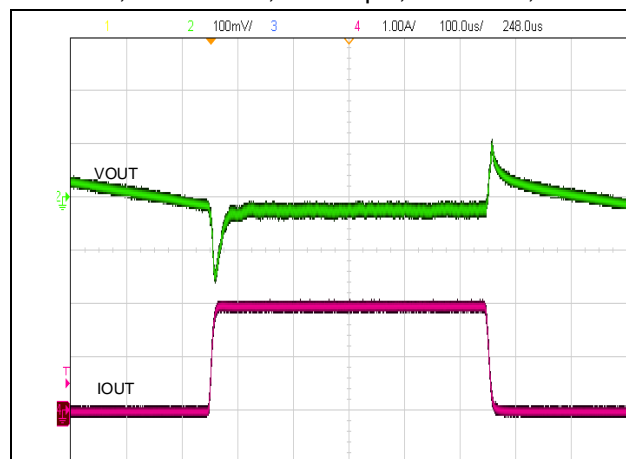
Figure 29. Load Transient
