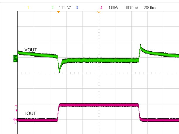
Figure 30. Load Transient
