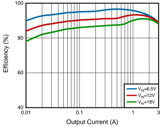
Figure 13. 5.0V Output Efficiency(DCR=27mΩ)
