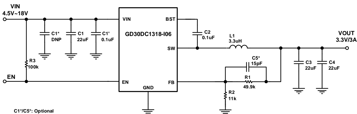
Figure 11. 3.3V, 3A Reference Design
