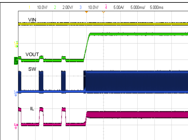
Figure 26. SCP Recovery
