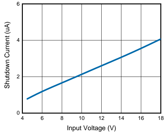
Figure 2. Shutdown Current vs. Input Voltage
