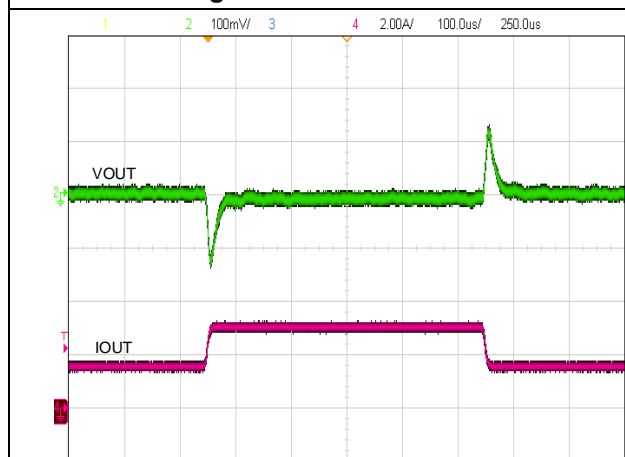
Figure 27. Load Transient
