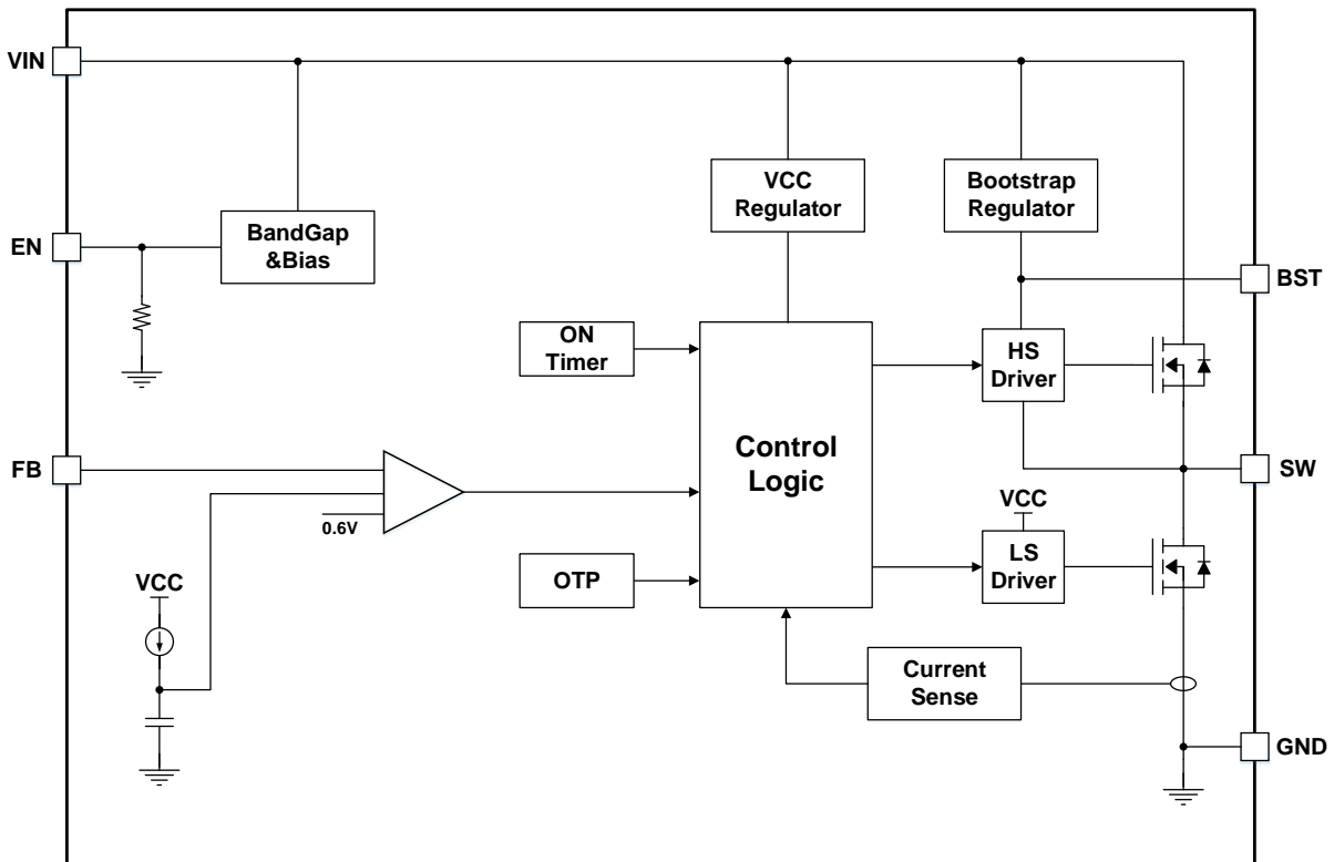
Figure 9. GD30DC1318-I06 Functional Block Diagram
