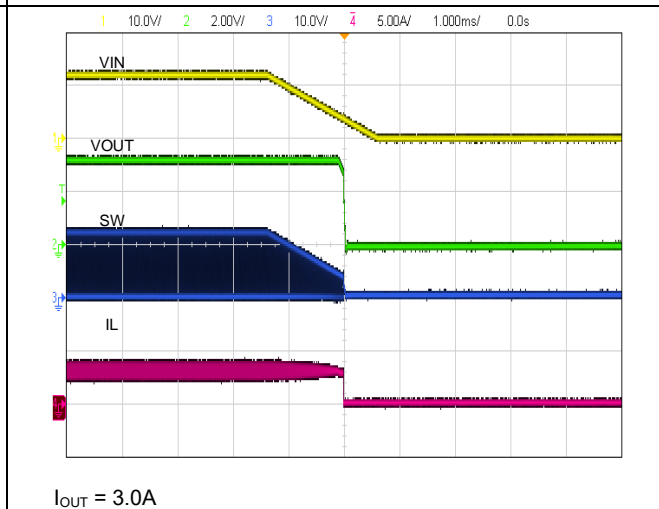
Figure 24. VIN ShutDown with Load
