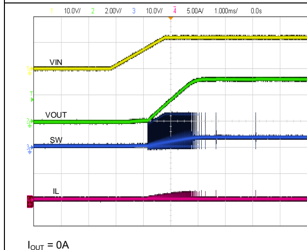
Figure 21. VIN StartUp without Load
