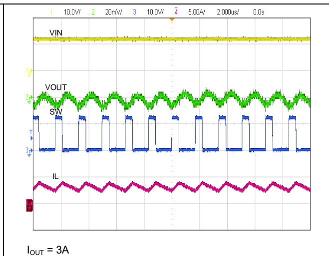
Figure 20. Output Ripple
