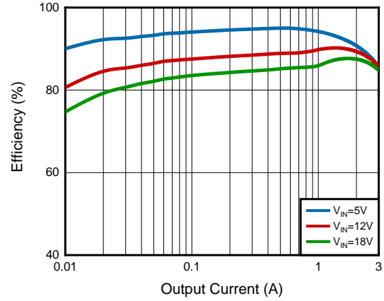
Figure 14. 3.3V Output Efficiency(DCR=20mΩ)
