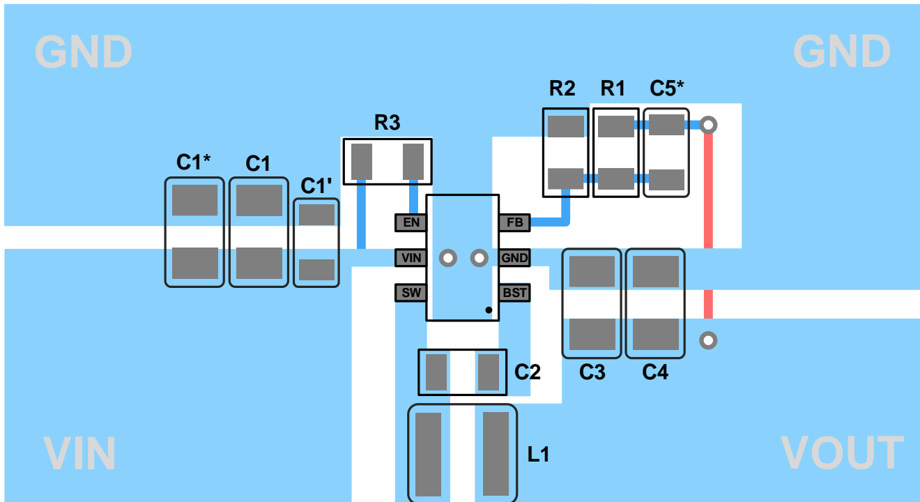
Figure 30. Typical GD30DC1318-I06 Example Layout
