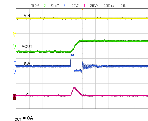
Figure 19. Output Ripple
