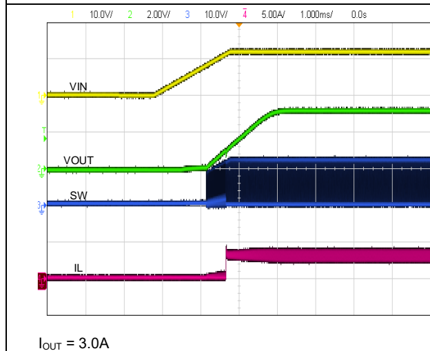
Figure 23. VIN StartUp with Load
