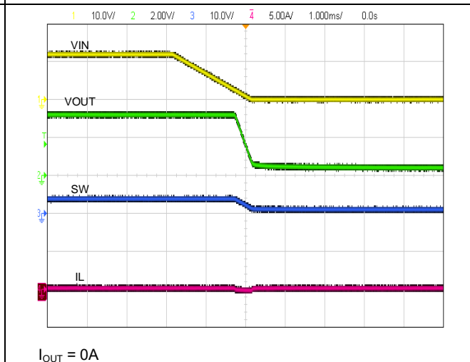
Figure 22. VIN ShutDown without Load
