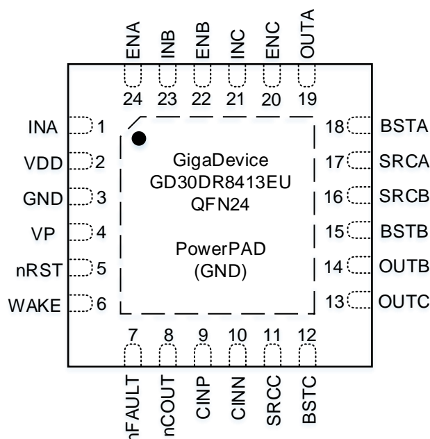
Figure 4-2 GD30DR8413x QFN24 Pinouts
