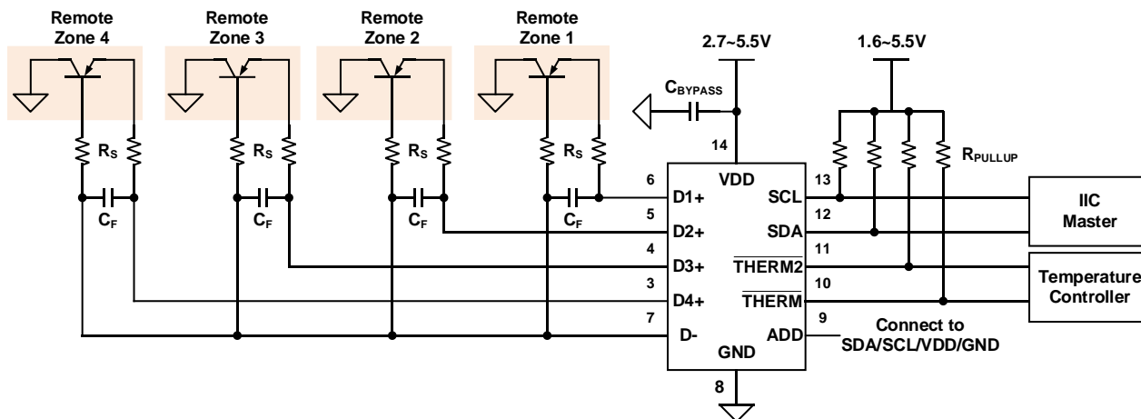
Figure 7. Diagram of GD30TS304T's Typical Connection
