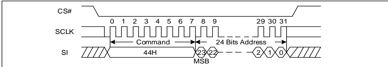
Figure 76 Erase Security Registers command Sequence Diagram (SPI)
