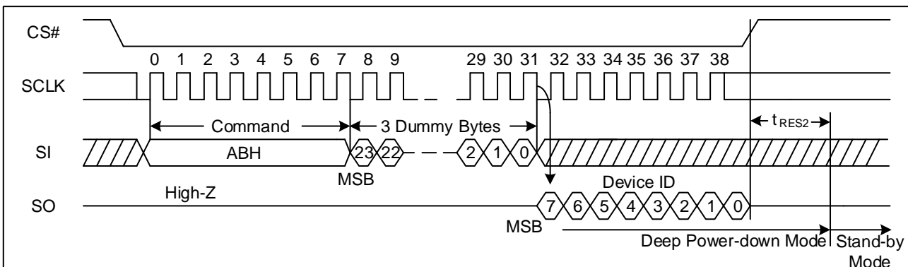
Figure 65. Release Power-Down/Read Device ID Sequence Diagram (SPI)
