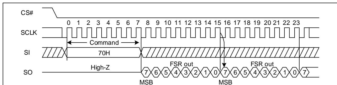
Figure 29 Read Flag Status Register Sequence Diagram (SPI)
