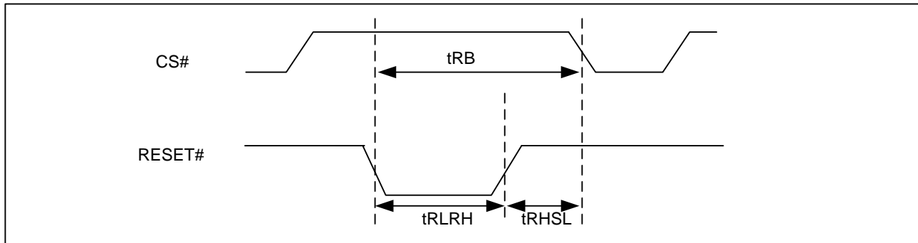
Figure 102. RESET Timing
