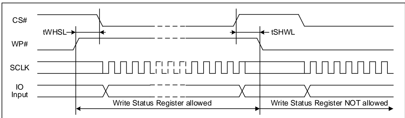
Figure 101. WP# Timing
