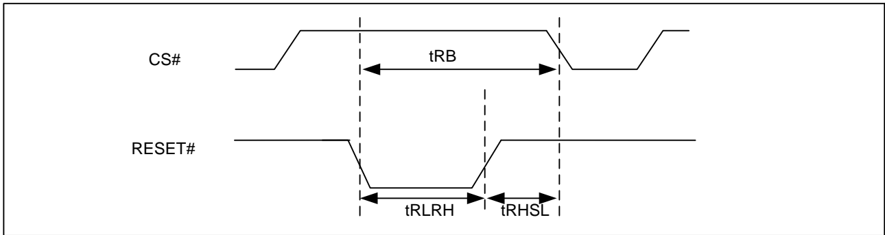
Figure 102. RESET Timing
