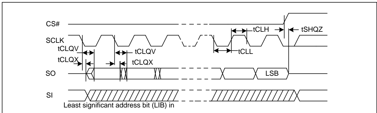
Figure 99. Output Timing
