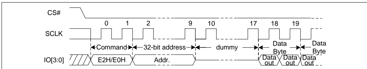
Figure 90 Read NL Register/VL Register Sequence (QPI)
