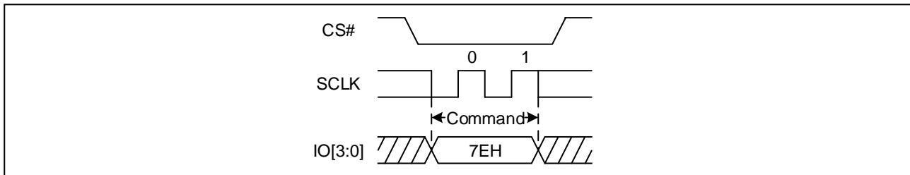
Figure 80 Global Block/Sector Lock Sequence Diagram (QPI)
