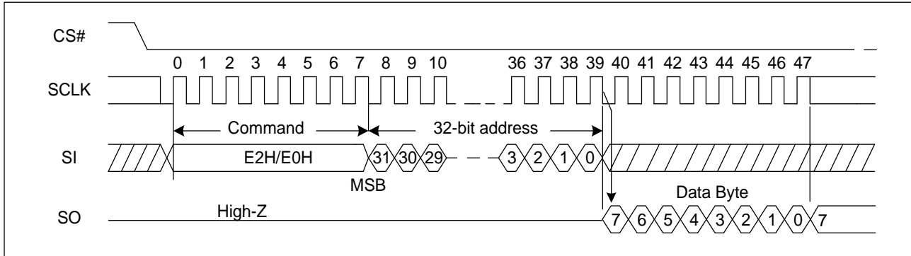
Figure 89 Read NL Register/VL Register Sequence Diagram (SPI)
