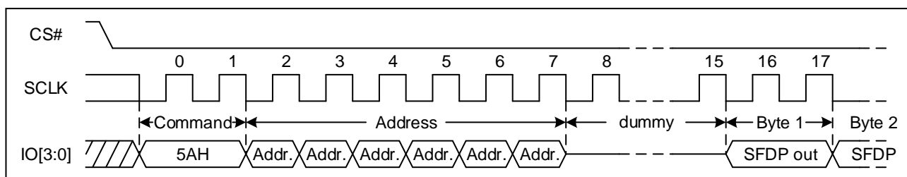
Figure 94 Read Serial Flash Discoverable Parameter command Sequence Diagram (QPI)
