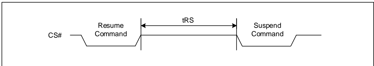
Figure 100. Resume to Suspend Timing Diagram
