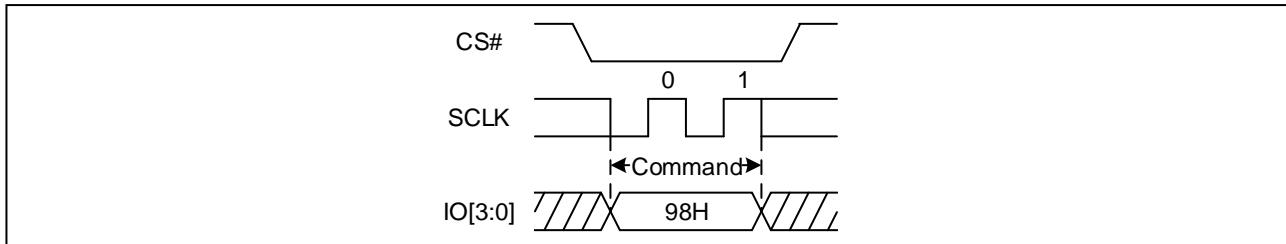
Figure 82 Global Block/Sector Unlock Sequence Diagram (QPI)
