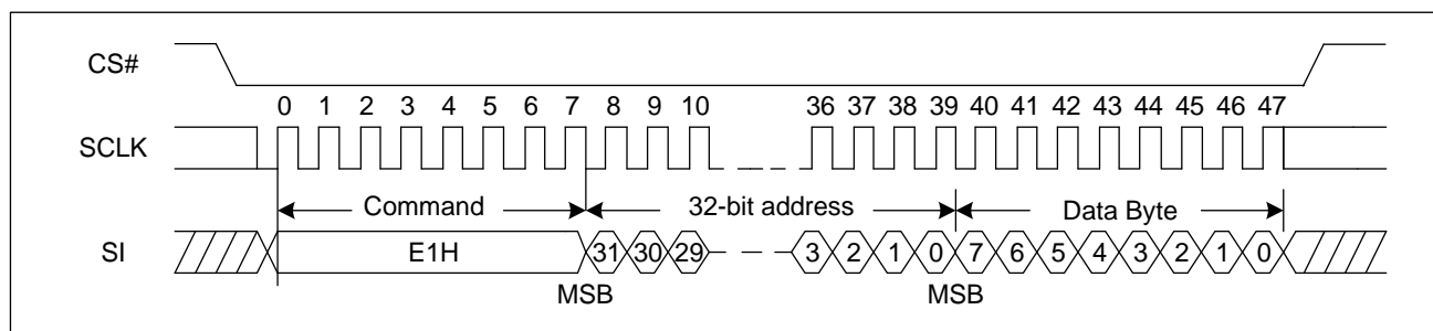
Figure 87 Write VL Register Sequence Diagram (SPI)
