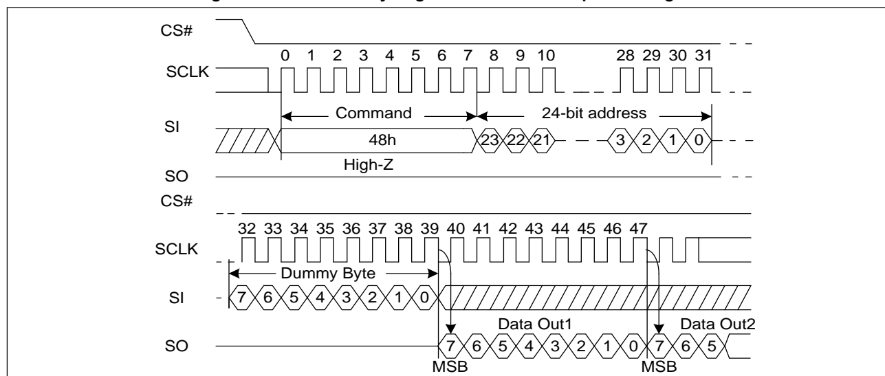
Figure 61. Read Security Registers command Sequence Diagram
