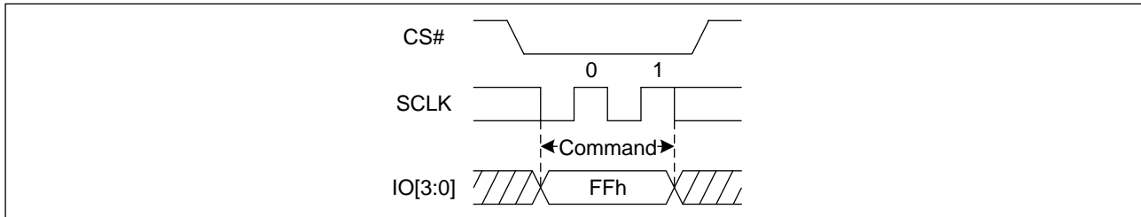
Figure 75. Disable QPI mode command Sequence Diagram
