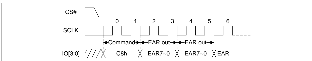
Figure 16. Read Extended Register Sequence Diagram (QPI)
