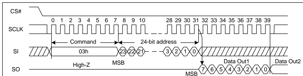
Figure 23. Read Data Bytes Sequence Diagram
