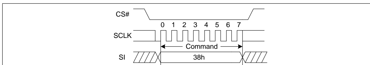
Figure 72. Enable QPI mode command Sequence Diagram
