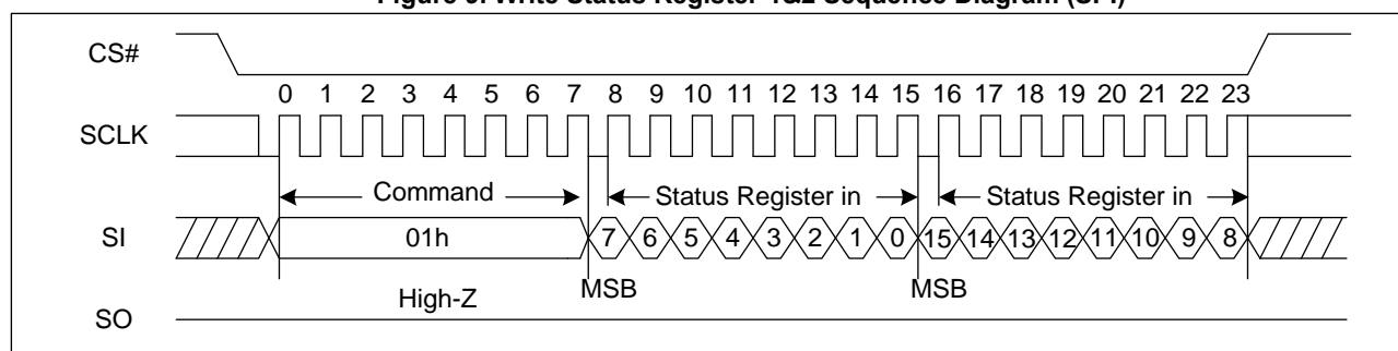
Figure 9. Write Status Register-1&2 Sequence Diagram (SPI)
