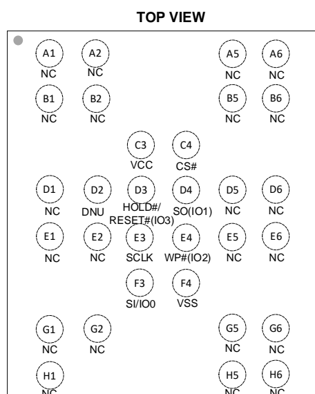
Figure 1. Connection Diagram for WLCSP package
