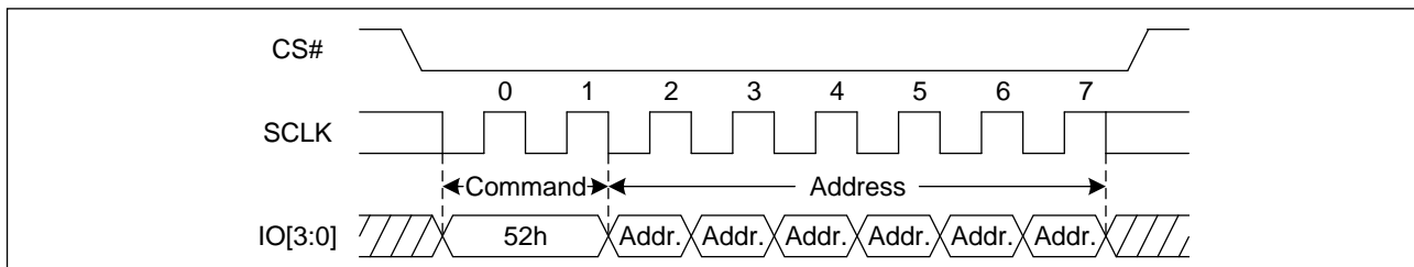
Figure 43. 32KB Block Erase Sequence Diagram (QPI)
