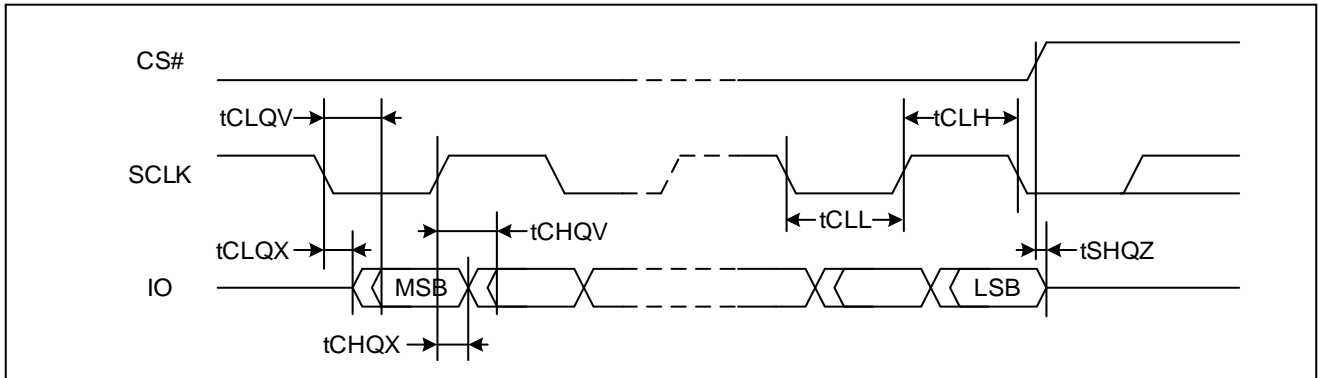
Figure 82. Serial Output Timing (DTR)
