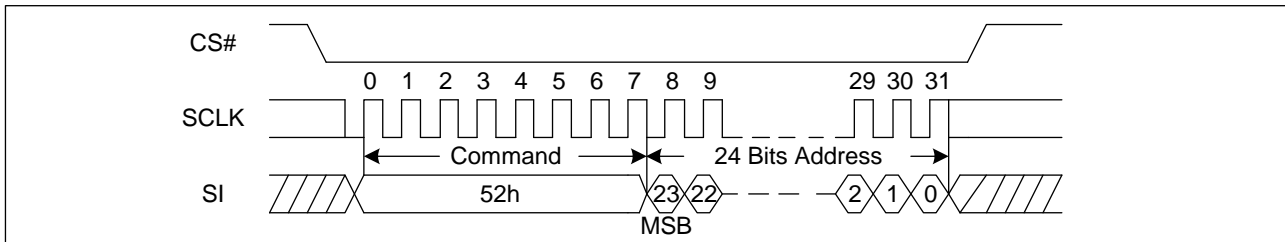
Figure 42. 32KB Block Erase Sequence Diagram (SPI)
