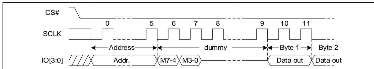
Figure 30. Quad I/O Fast Read Sequence Diagram ((M5-4) = (1, 0))
