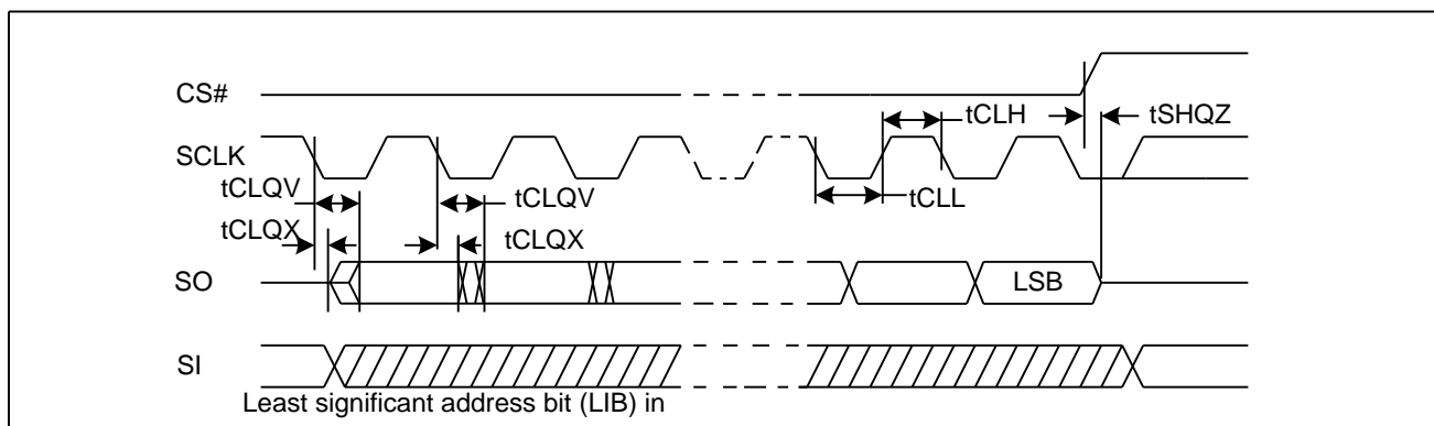
Figure 80. Output Timing
