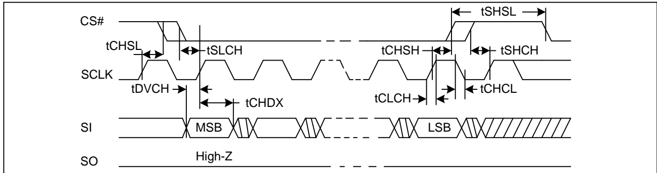
Figure 79. Input Timing
