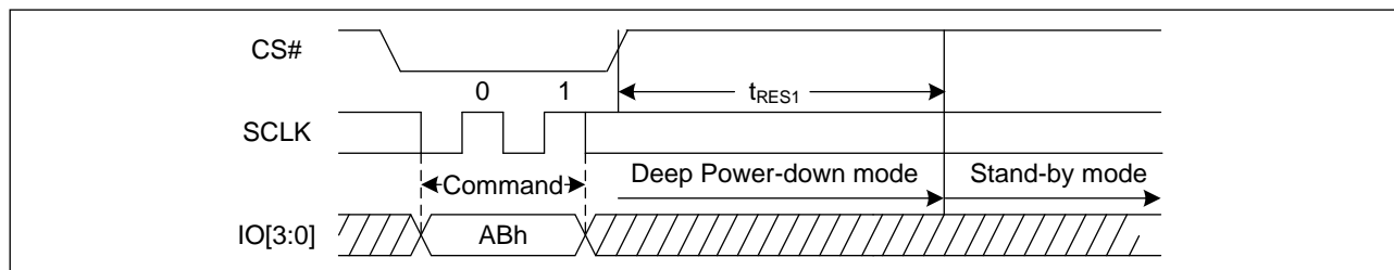
Figure 69. Release Power-Down Sequence Diagram (QPI)
