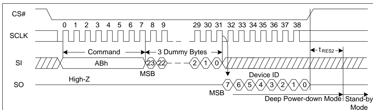
Figure 70. Release Power-Down/Read Device ID Sequence Diagram (SPI)
