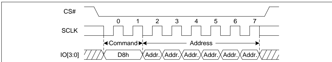
Figure 45. 64KB Block Erase Sequence Diagram (QPI)
